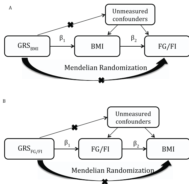
Figure 6. Mendelian randomization analysis to explore causality between BMI and FG/FI. (A) IV estimator is calculated as the beta coefficient from the association of GRS_{BMI} with FG or FI divided by the beta coefficient from the association of GRS_{BMI} with BMI (IV estimator = 0.31 pmol/l/BMI unit). The IV estimator is equivalent to what is seen when FI is regressed on BMI. These results are supportive of a causal, non-confounded relationship. (B) The relationship of FG or FI with BMI.
